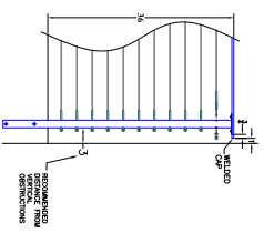
TYPICAL END CONDITION (A)
