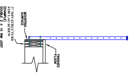
SECTION VIEW (C)
