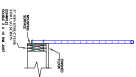
SECTION VIEW (C)
