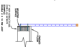
SECTION VIEW (C)
