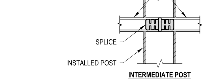
C FITTING INSTALLATION - OLYMPUS SPLICE DETAIL
