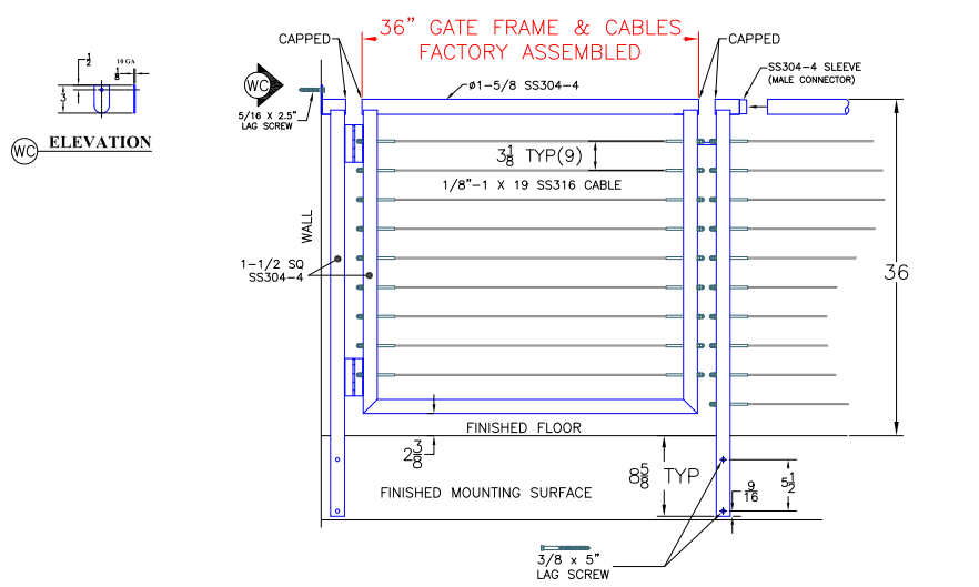
① SIDE MOUNT 36" SYSTEM WITH ROUND TOP RAIL AT WALL
