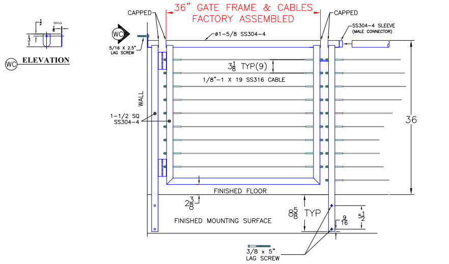
① SIDE MOUNT 36" SYSTEM WITH ROUND TOP RAIL AT WALL
