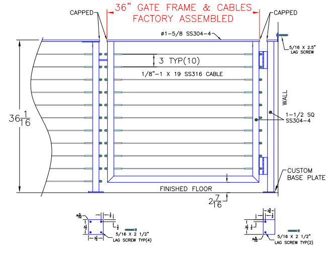
② TOP MOUNT 36" SYSTEM WITH FLAT TOP RAIL AT WALL
