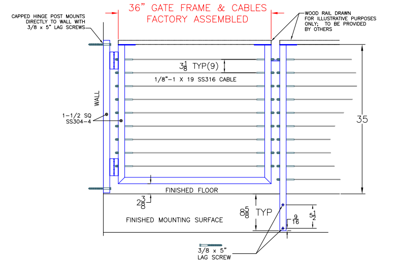
① SIDE MOUNT 36" SYSTEM WITH WOOD TOP RAIL AT WALL
