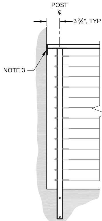
1 END POST - WALL CONNECTION ELEVATION
